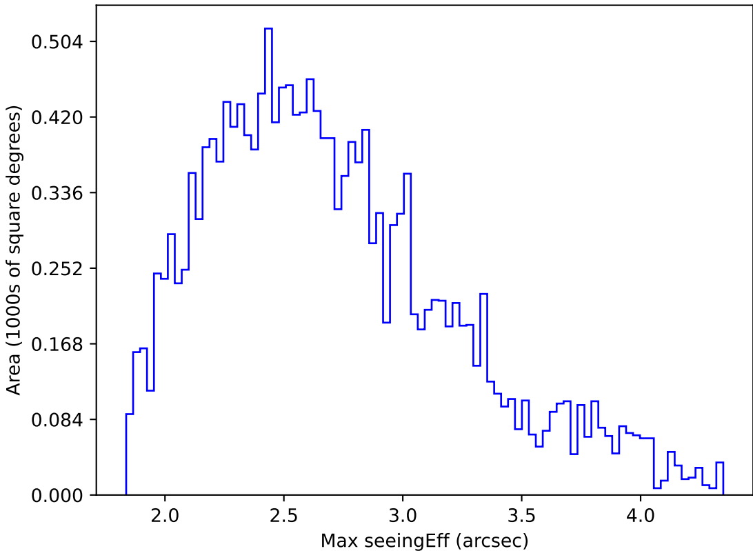
ddf_acor_sf20_lsf40_lsr50_v3.4_10yrs WFD r band: Max seeingEff
