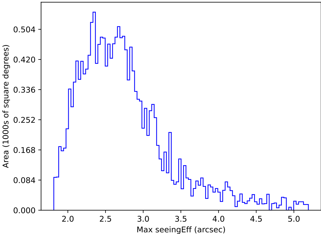
ddf_acor_sf20_lsf40_lsr50_v3.4_10yrs WFD i band: Max seeingEff
