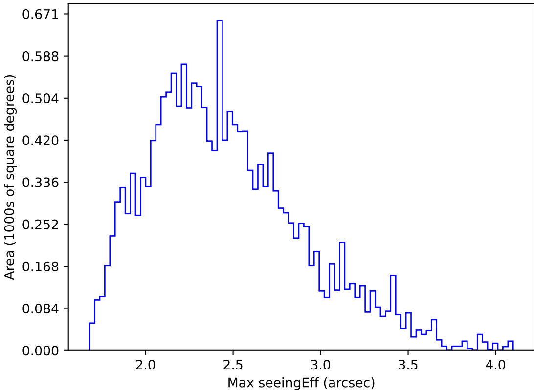
ddf_acor_sf20_lsf40_lsr50_v3.4_10yrs WFD g band: Max seeingEff
