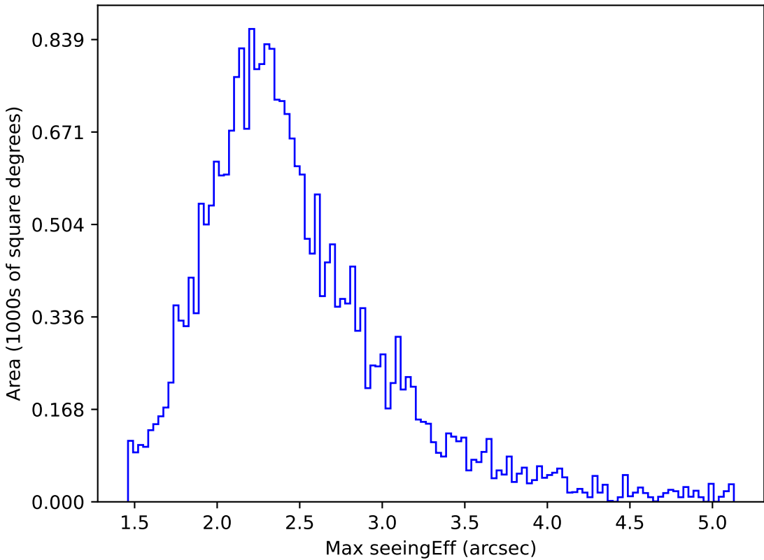
ddf_acor_sf20_lsf40_lsr50_v3.4_10yrs All sky z band: Max seeingEff
