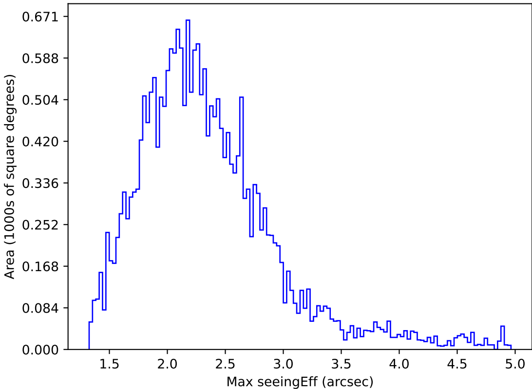
ddf_acor_sf20_ls40_lsr50_v3.4_10yrs All sky y band: Max seeingEff
