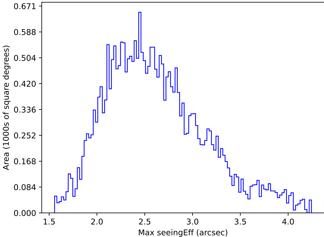
ddf_acor_sf20_lsf40_lsr50_v3.4_10yrs All sky r band: Max seeingEff
