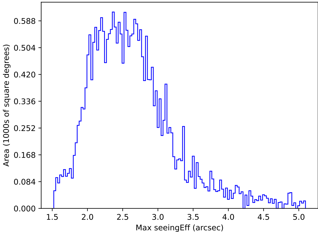
ddf_acor_sf20_lsf40_lsr50_v3.4_10yrs All sky i band: Max seeingEff
