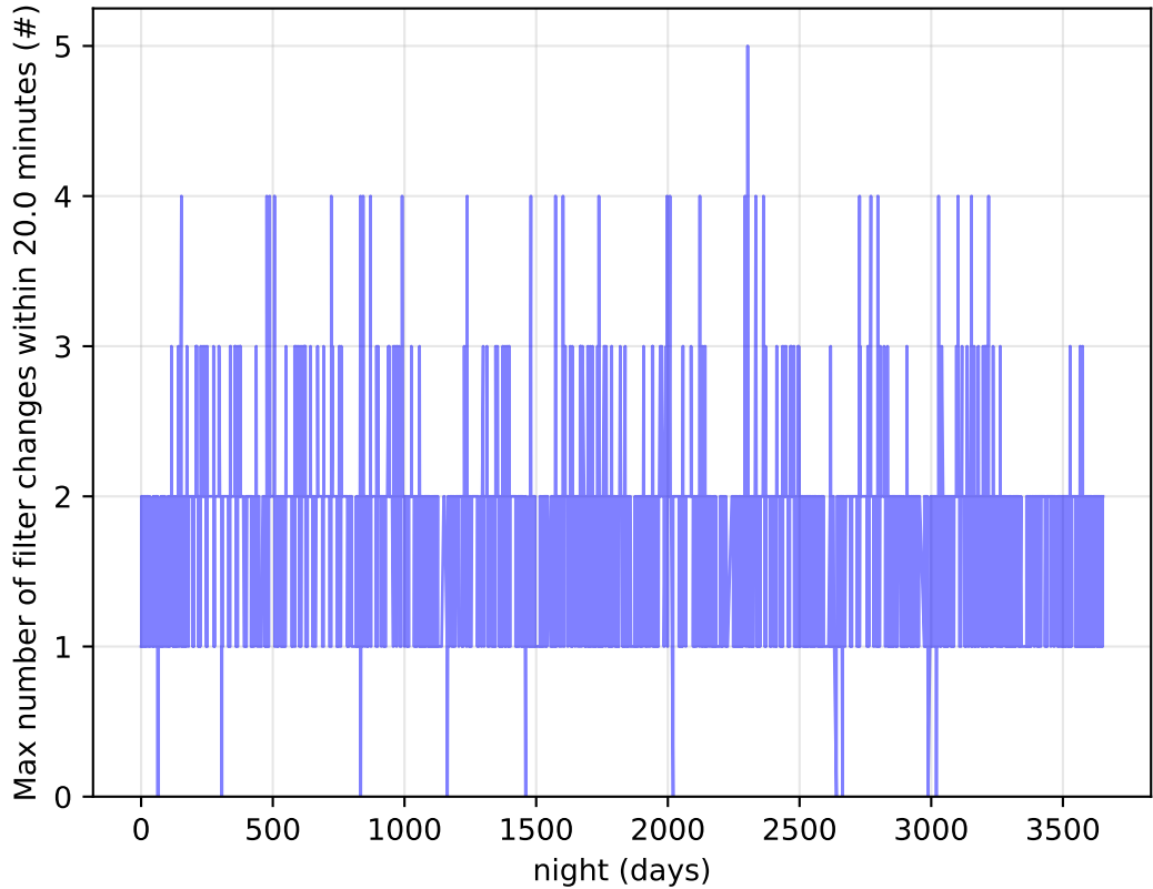
ddf_acor_sf20_Isf40_Isr50_v3.4_10yrs Per Night: Max number of filter changes within 20.0 minutes
