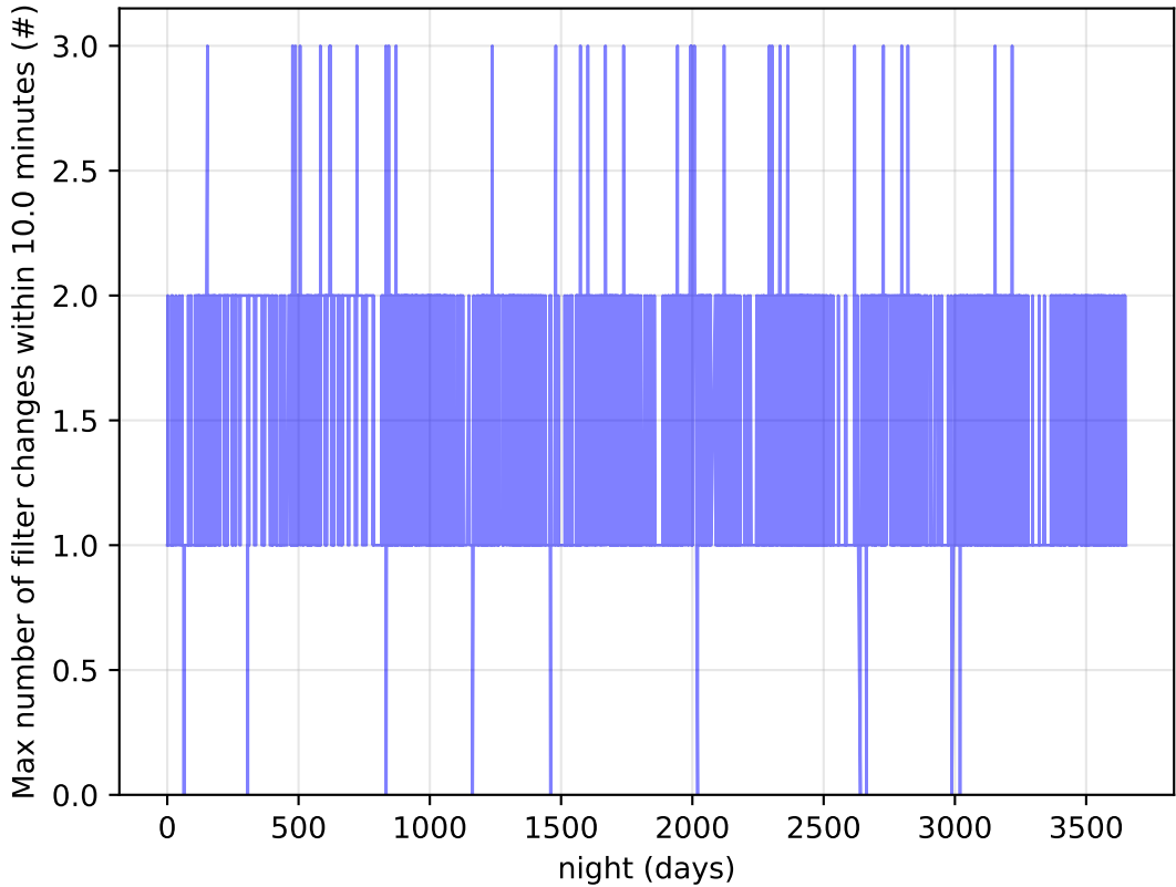
ddf_acor_sf20_Isf40_Isr50_v3.4_10yrs Per Night: Max number of filter changes within 10.0 minutes
