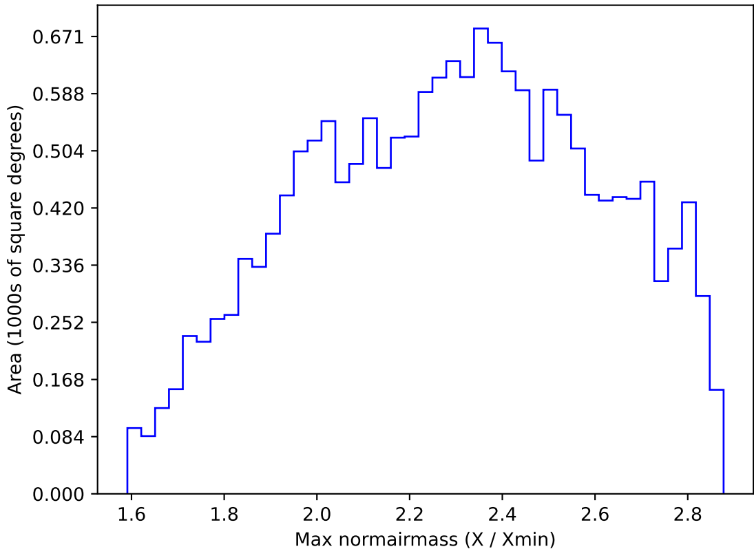
ddf_acor_sf20_lsf40_lsr50_v3.4_10yrs WFD i band: Max normairmass
