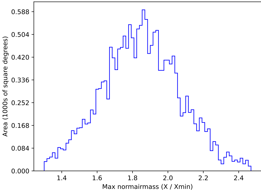
ddf_acor_sf20_lsf40_lsr50_v3.4_10yrs WFD g band: Max normairmass
