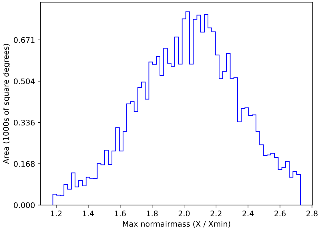
ddf_acor_sf20_lsf40_lsr50_v3.4_10yrs All sky y band: Max normairmass
