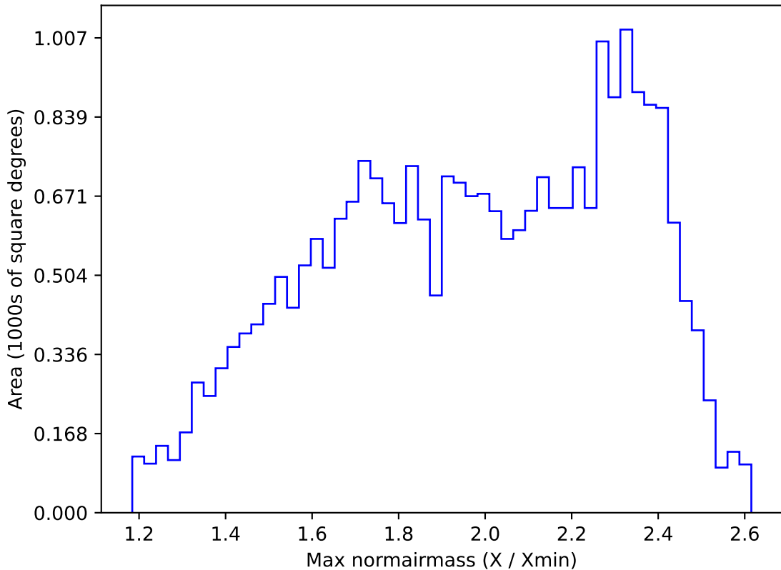
ddf_acor_sf20_lsf40_lsr50_v3.4_10yrs All sky r band: Max normairmass
