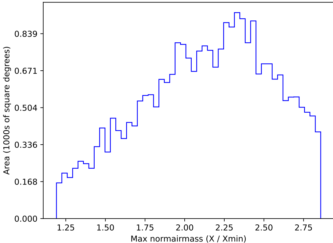
ddf_acor_sf20_lsf40_lsr50_v3.4_10yrs All sky i band: Max normairmass
