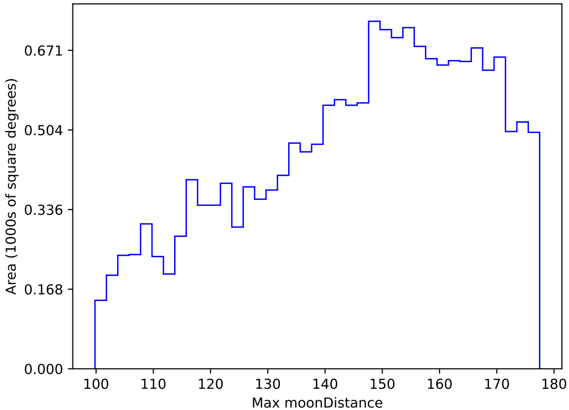
ddf_acor_sf20_ls40_lsr50_v3.4_10yrs WFD y band: Max moonDistance
