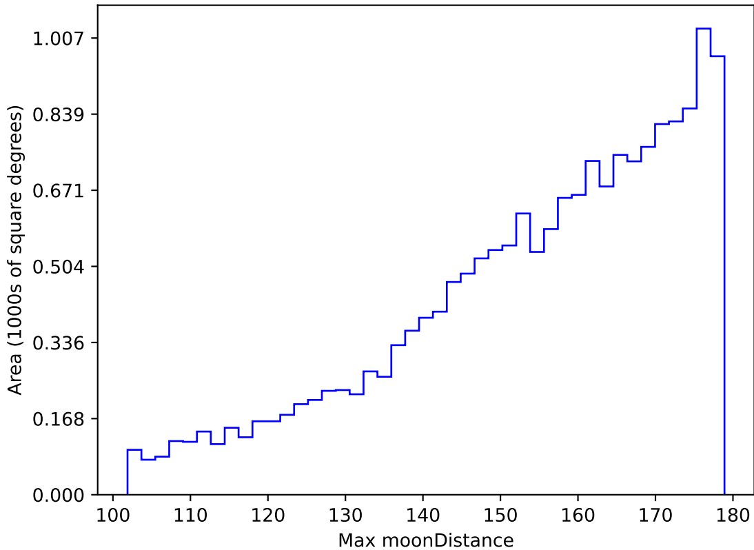
ddf_acor_sf20_lsf40_lsr50_v3.4_10yrs WFD u band: Max moonDistance
