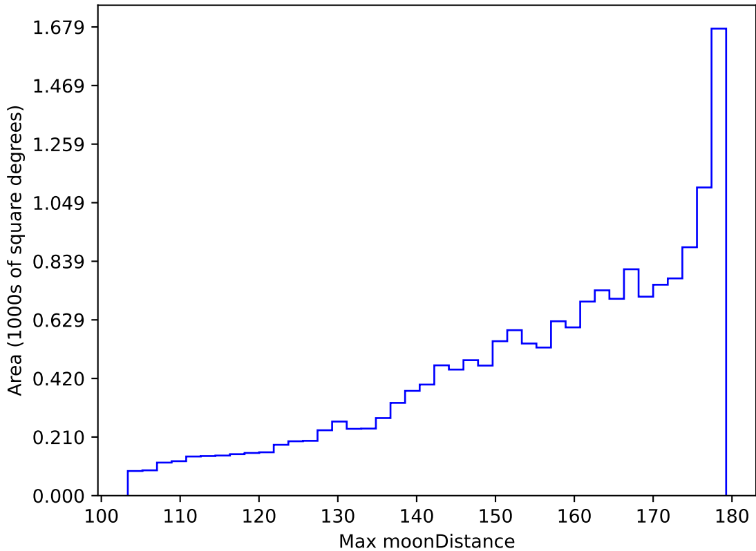
ddf_acor_sf20_lsf40_lsr50_v3.4_10yrs WFD r band: Max moonDistance
