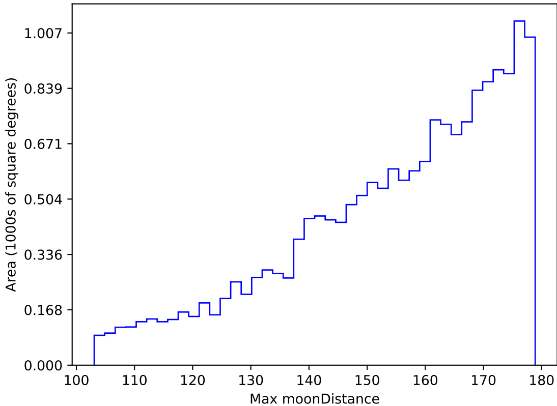
ddf_acor_sf20_lsf40_lsr50_v3.4_10yrs WFD g band: Max moonDistance
