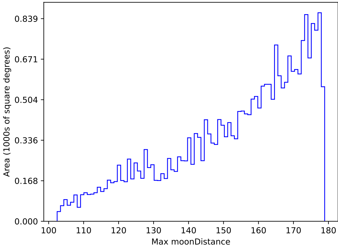
ddf_acor_sf20_lsf40_lsr50_v3.4_10yrs All sky z band: Max moonDistance
