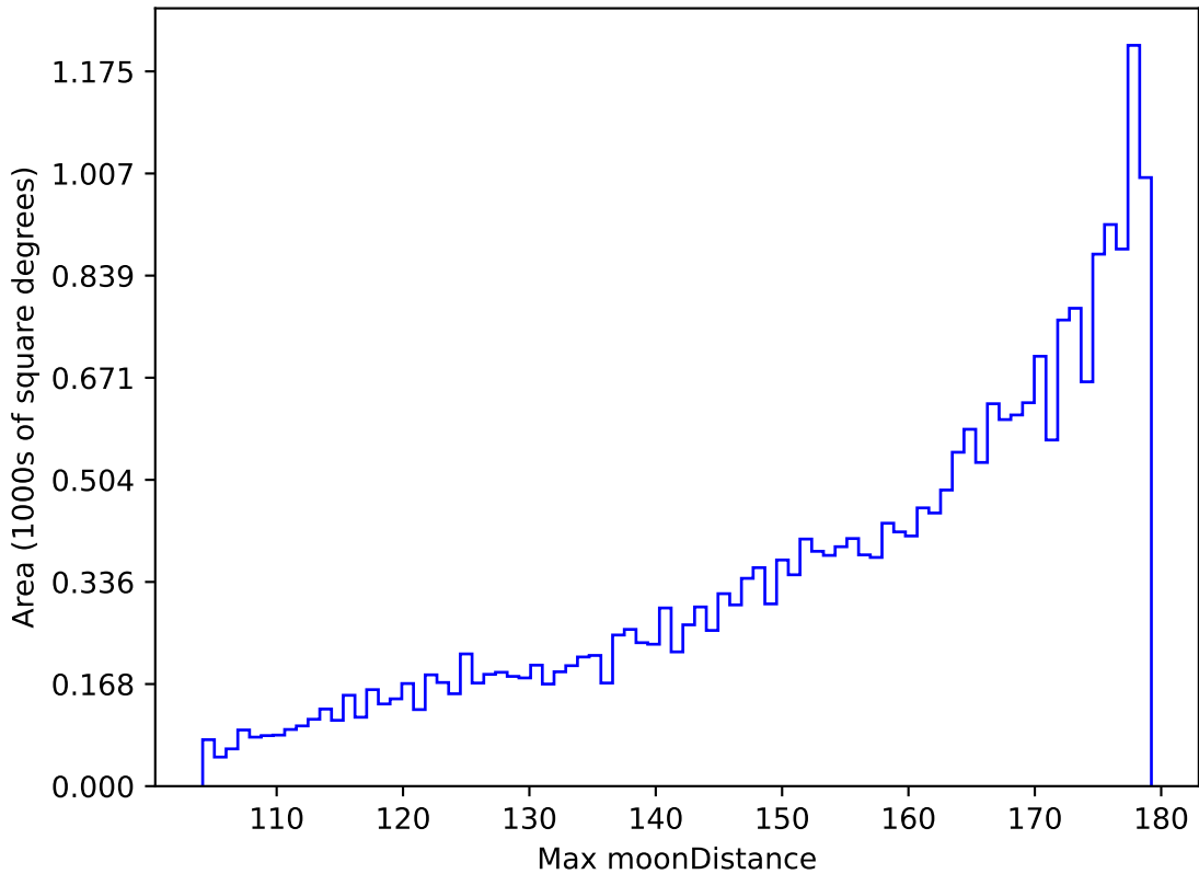
ddf_acor_sf20_lsf40_lsr50_v3.4_10yrs All sky r band: Max moonDistance
