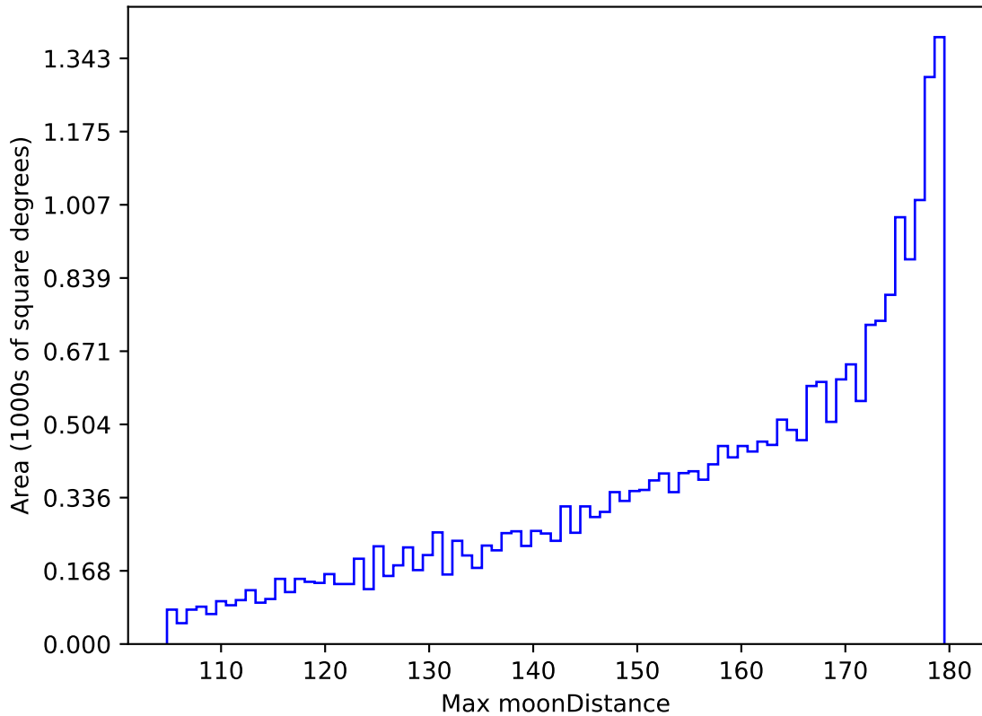
ddf_acor_sf20_lsf40_lsr50_v3.4_10yrs All sky all bands: Max moonDistance
