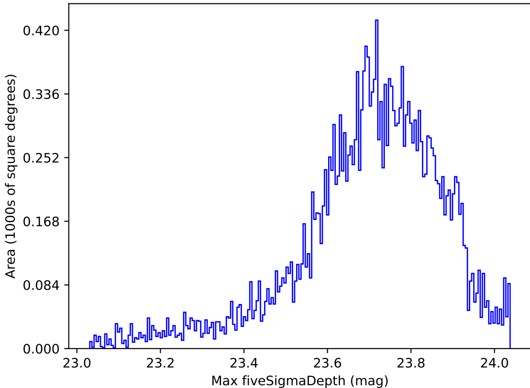
ddf_acor_sf20_lsf40_lsr50_v3.4_10yrs All sky u band: Max fiveSigmaDepth
