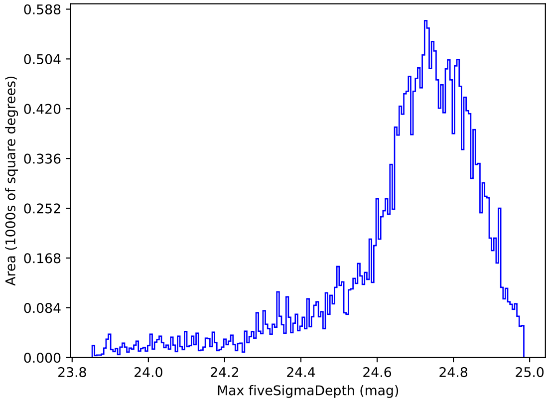
ddf_acor_sf20_lsf40_lsr50_v3.4_10yrs All sky r band: Max fiveSigmaDepth
