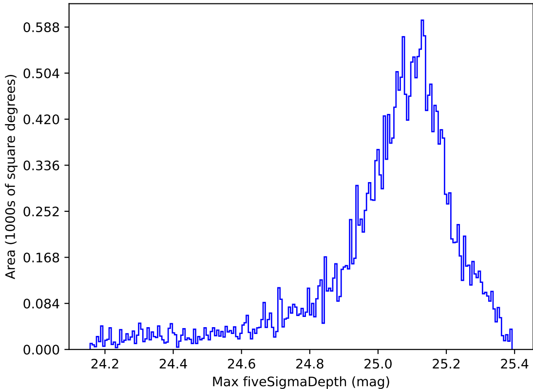
ddf_acor_sf20_lsf40_lsr50_v3.4_10yrs All sky g band: Max fiveSigmaDepth
