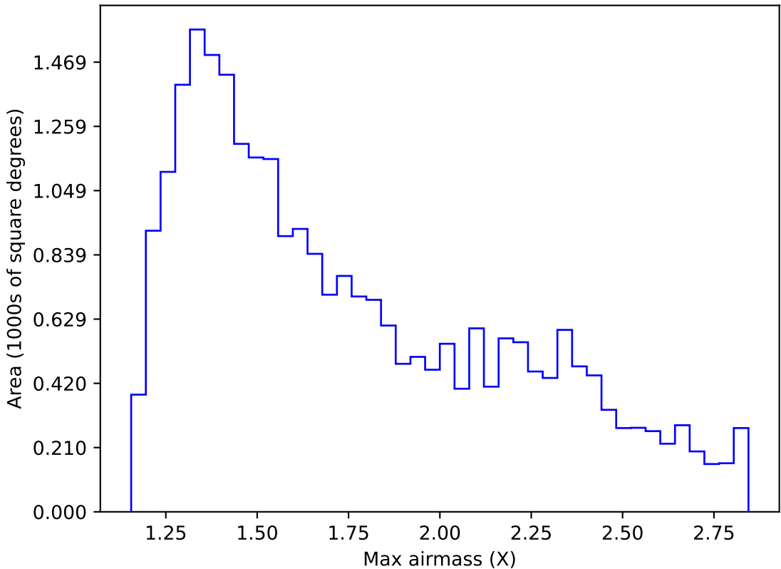
ddf_acor_sf20_lsf40_lsr50_v3.4_10yrs Yr 1 z band: Max airmass
