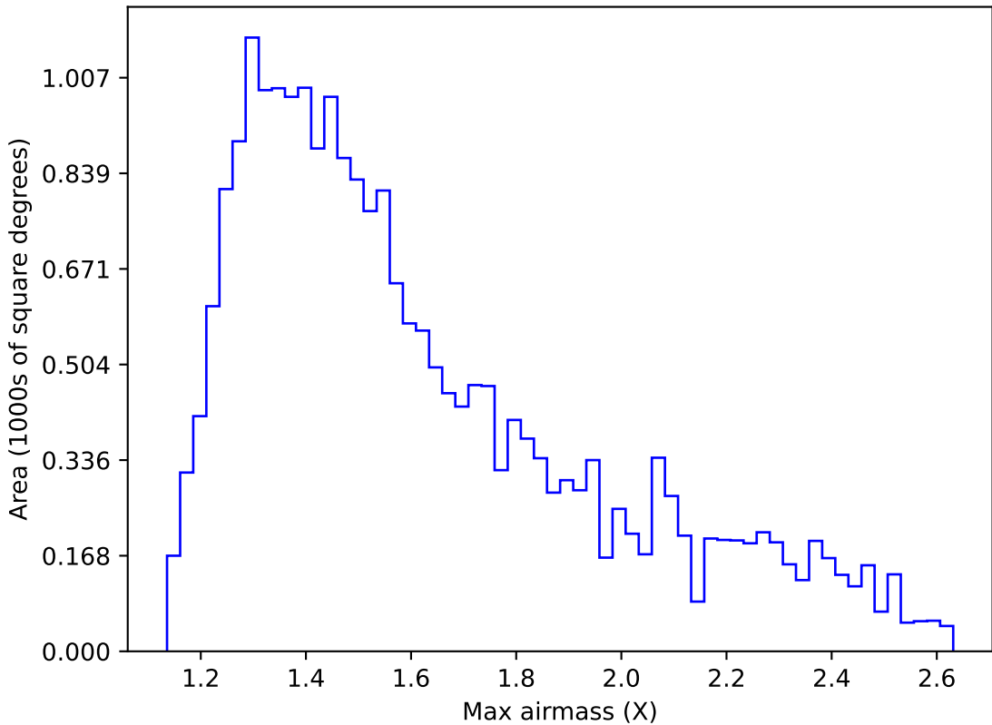
ddf_acor_sf20_lsf40_lsr50_v3.4_10yrs Yr 1 y band: Max airmass
