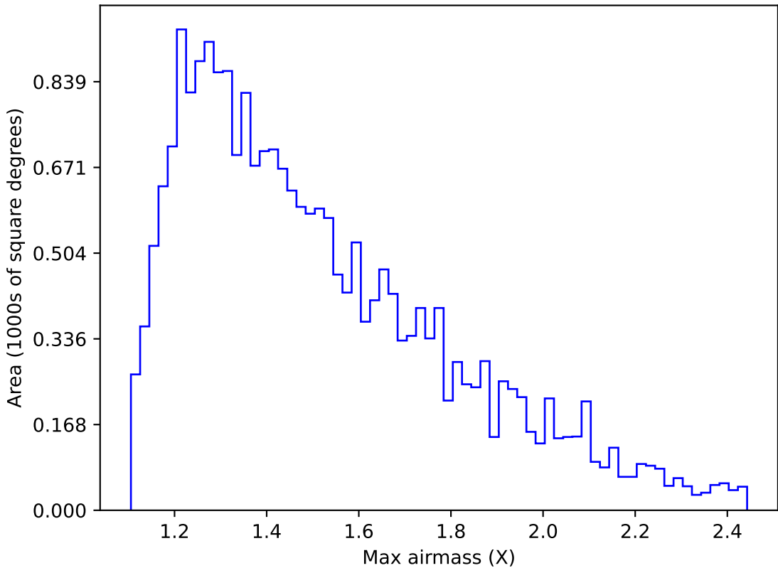
ddf_acor_sf20_lsf40_lsr50_v3.4_10yrs Yr 1 u band: Max airmass
