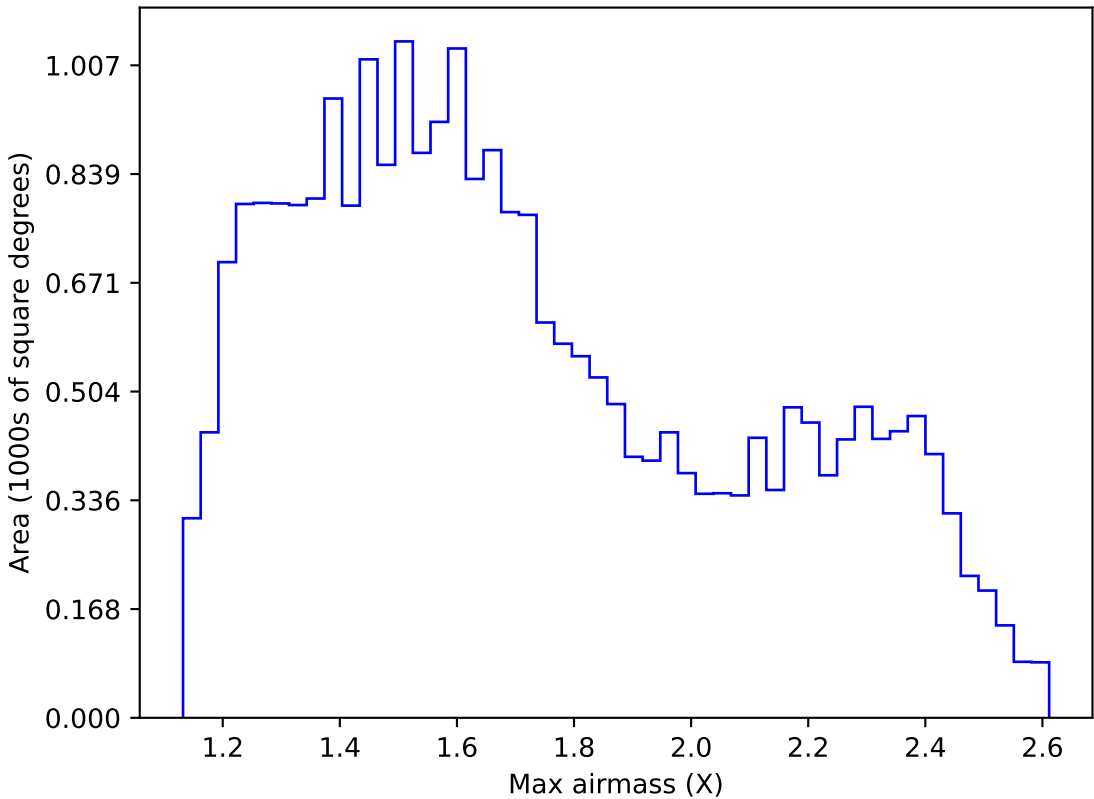
ddf_acor_sf20_ls40_lsr50_v3.4_10yrs Yr 1 r band: Max airmass
