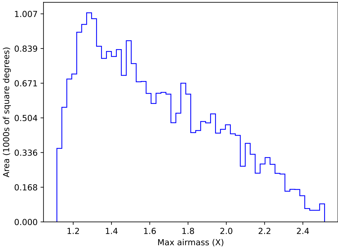
ddf_acor_sf20_lsf40_lsr50_v3.4_10yrs Yr 1 g band: Max airmass
