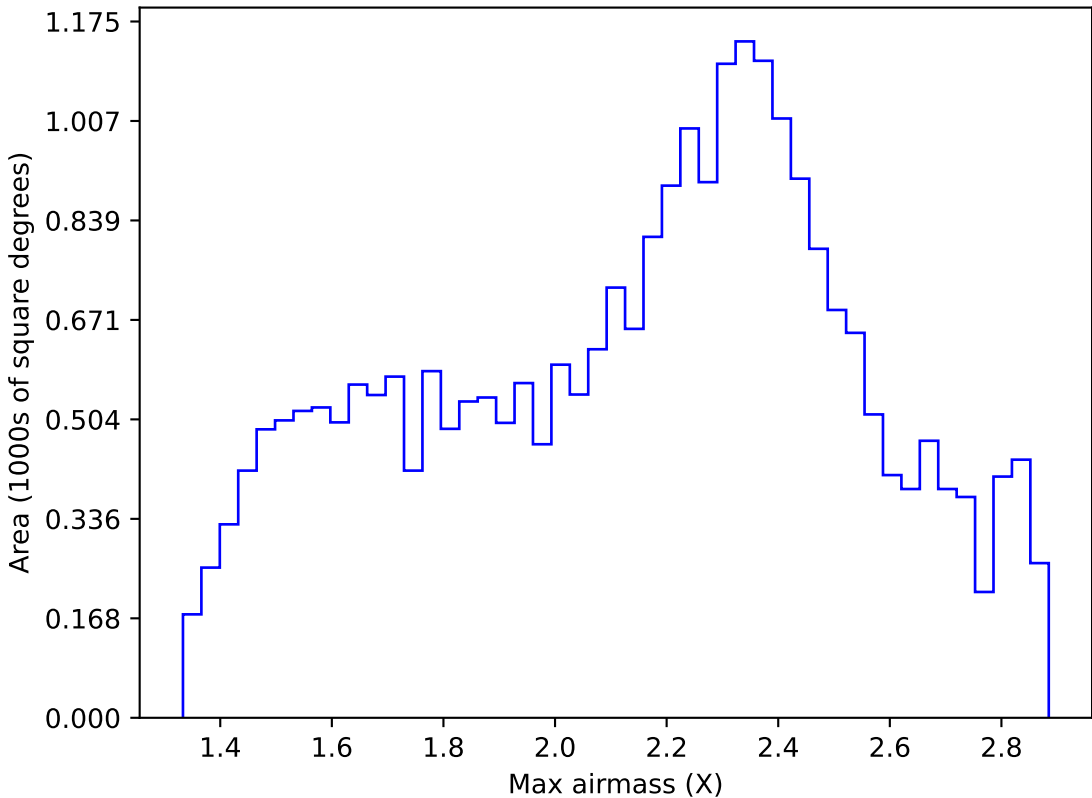
ddf_acor_sf20_lsf40_lsr50_v3.4_10yrs Yr 1 all bands: Max airmass
