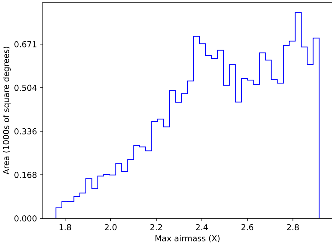
ddf_acor_sf20_lsf40_lsr50_v3.4_10yrs WFD z band: Max airmass
