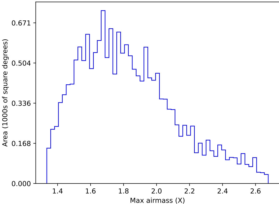
ddf_acor_sf20_lsf40_lsr50_v3.4_10yrs WFD u band: Max airmass
