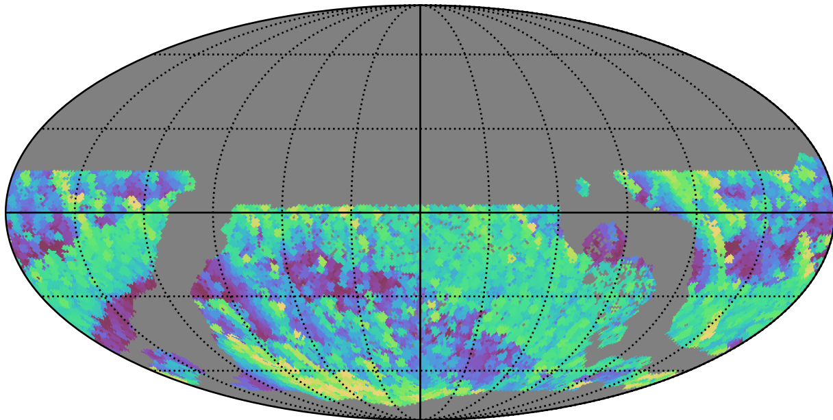
ddf_acor_sf20_lsf40_lsr50_v3.4_10yrs WFD r band: Max airmass
