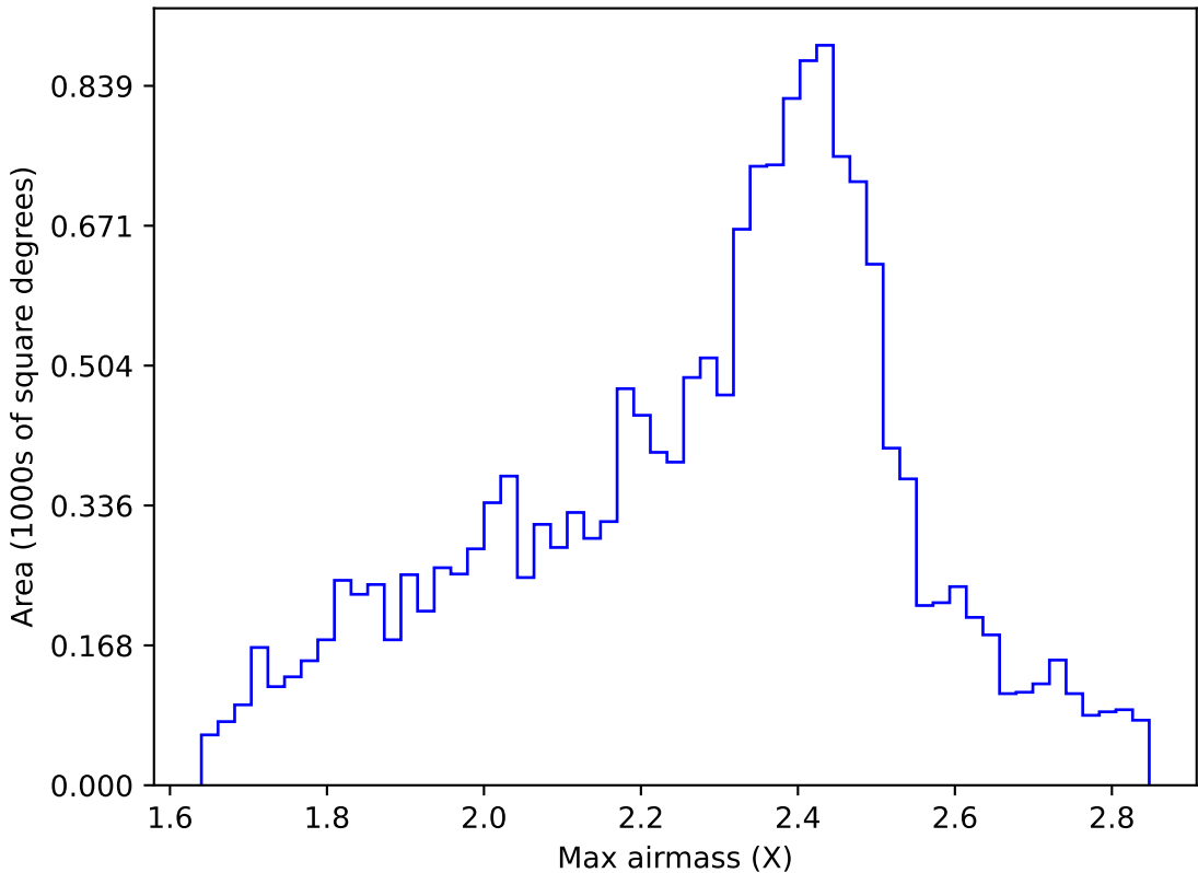
ddf_acor_sf20_lsf40_lsr50_v3.4_10yrs WFD r band: Max airmass
