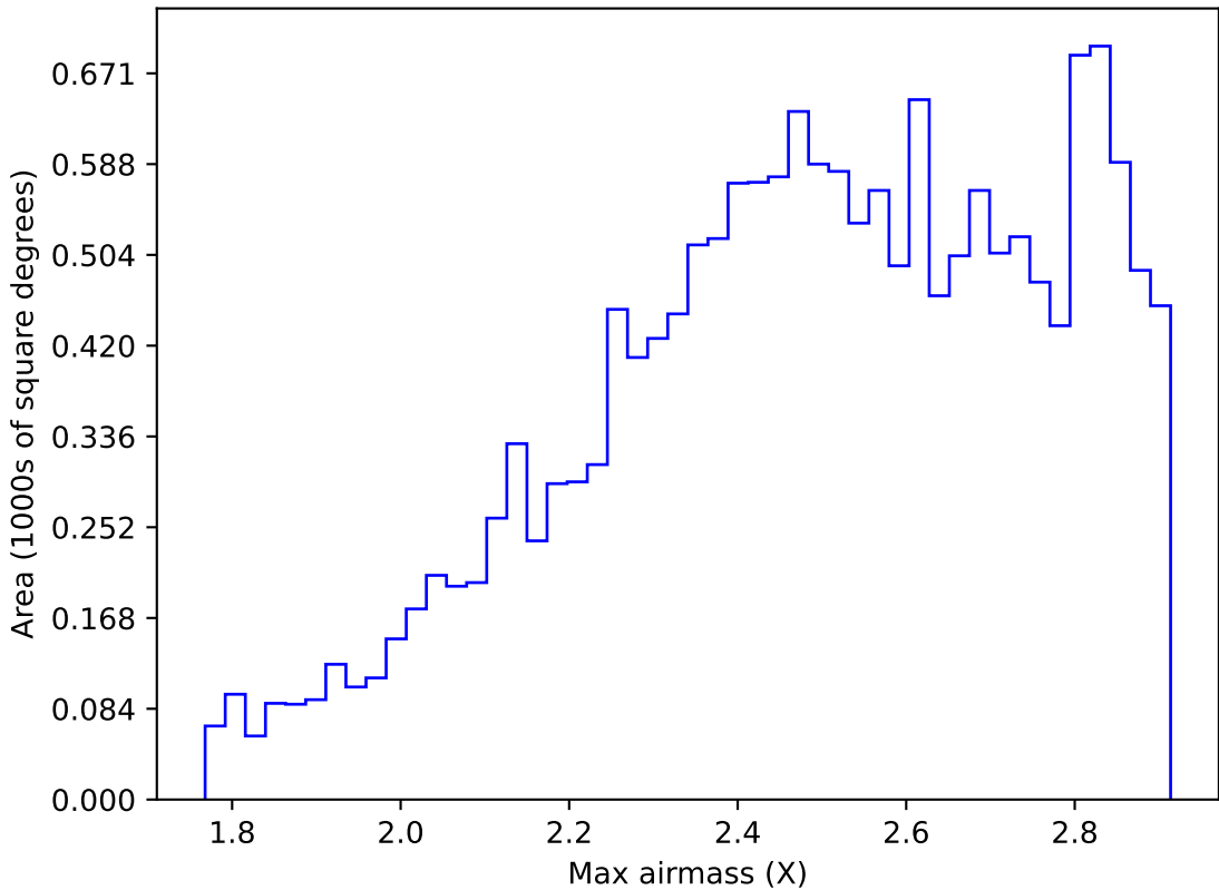
ddf_acor_sf20_lsf40_lsr50_v3.4_10yrs WFD i band: Max airmass
