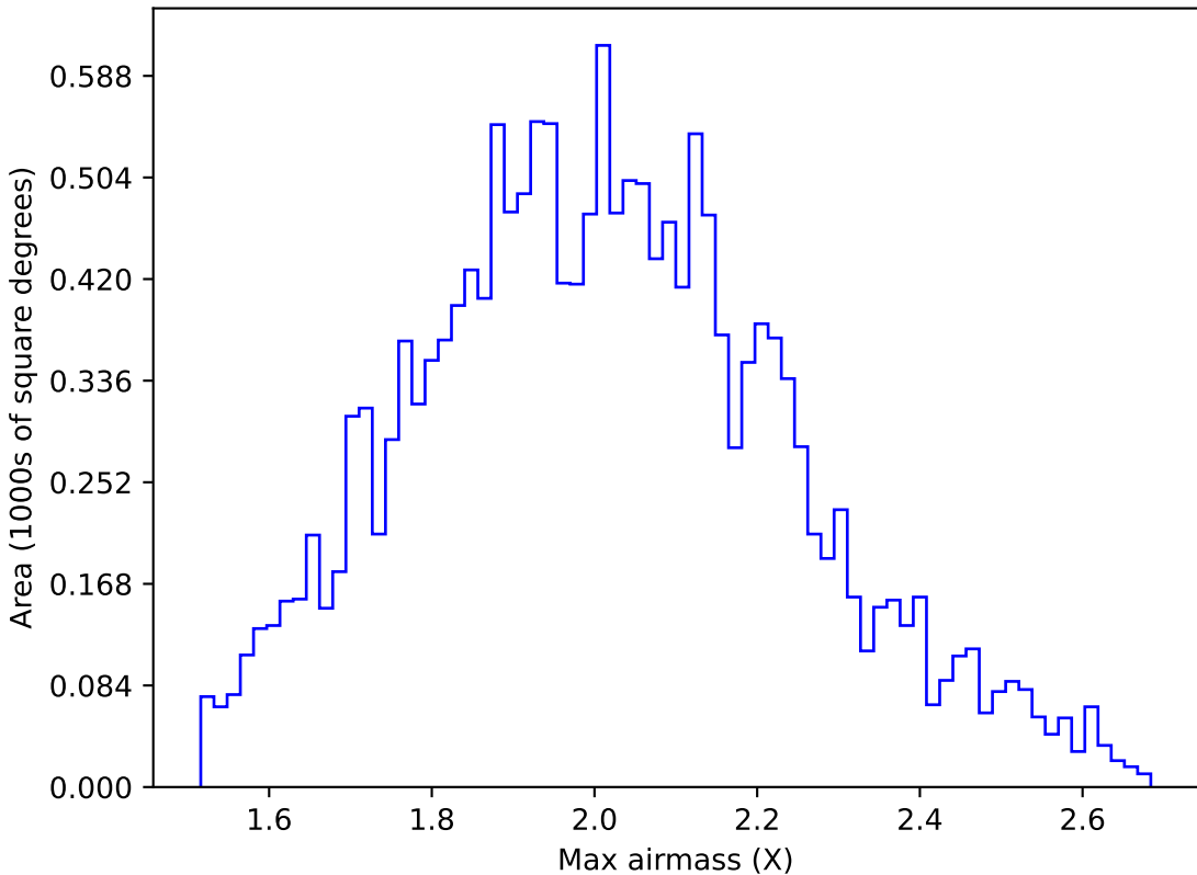
ddf_acor_sf20_lsf40_lsr50_v3.4_10yrs WFD g band: Max airmass
