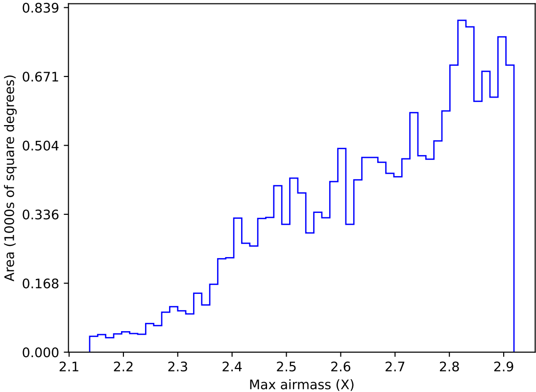
ddf_acor_sf20_lsf40_lsr50_v3.4_10yrs WFD all bands: Max airmass
