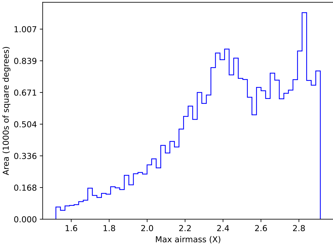
ddf_acor_sf20_lsf40_lsr50_v3.4_10yrs All sky z band: Max airmass
