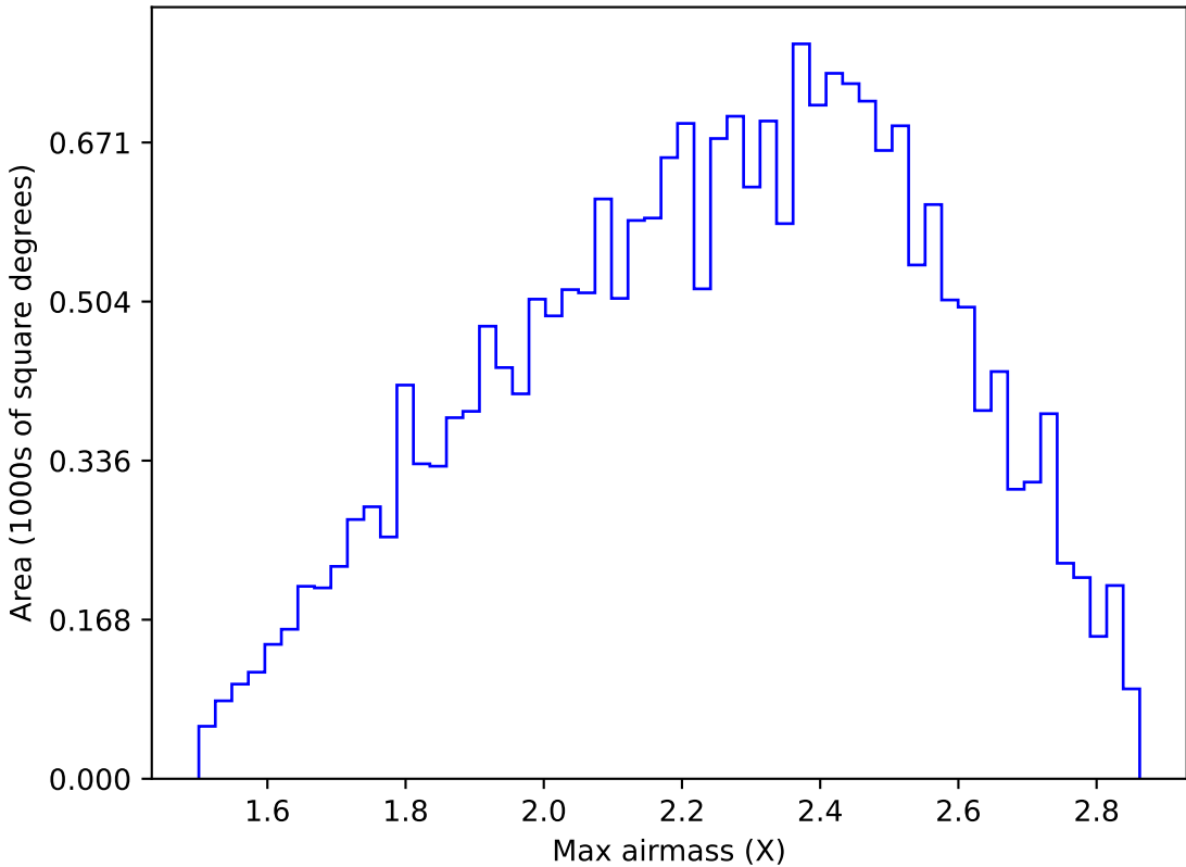
ddf_acor_sf20_lsf40_lsr50_v3.4_10yrs All sky y band: Max airmass
