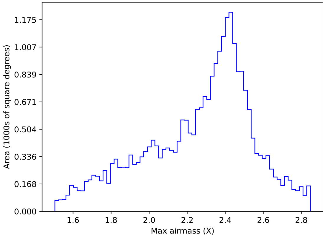
ddf_acor_sf20_lsf40_lsr50_v3.4_10yrs All sky r band: Max airmass
