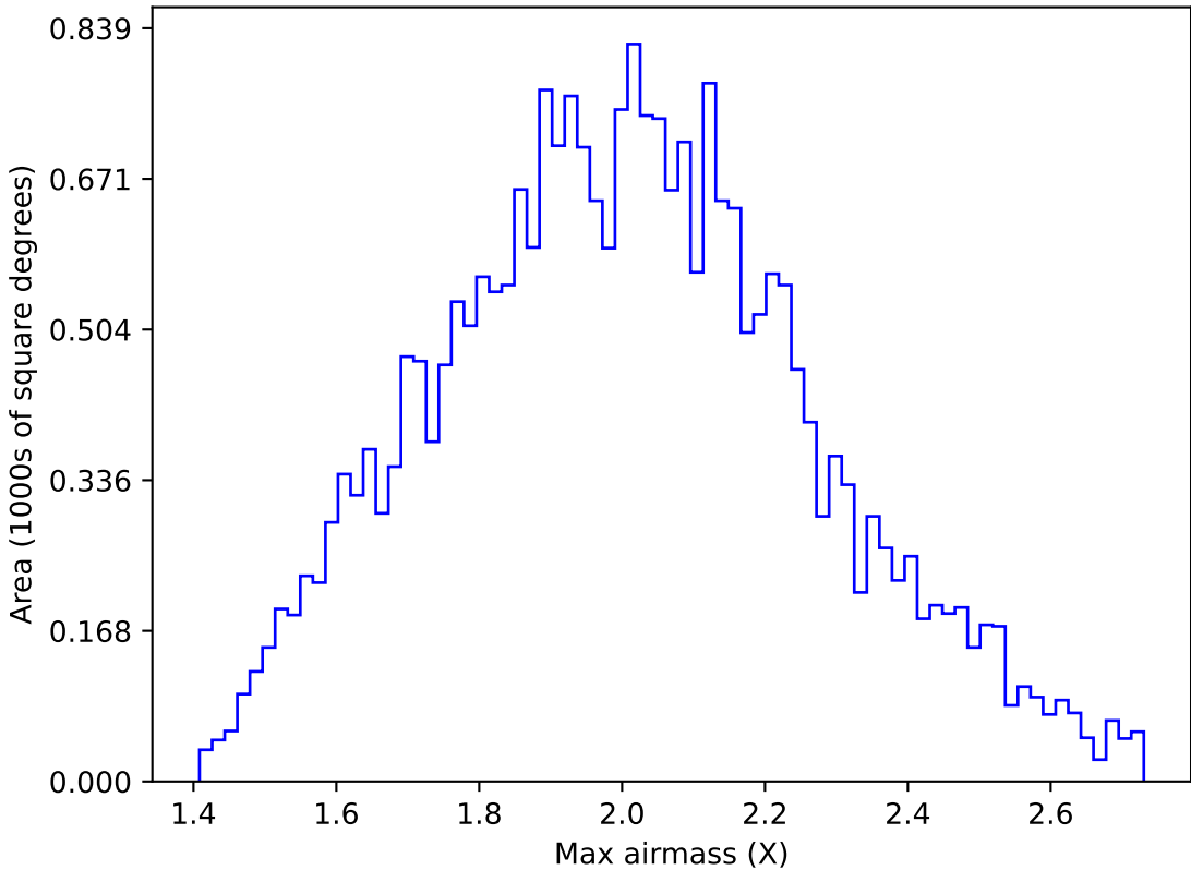
ddf_acor_sf20_lsf40_lsr50_v3.4_10yrs All sky g band: Max airmass
