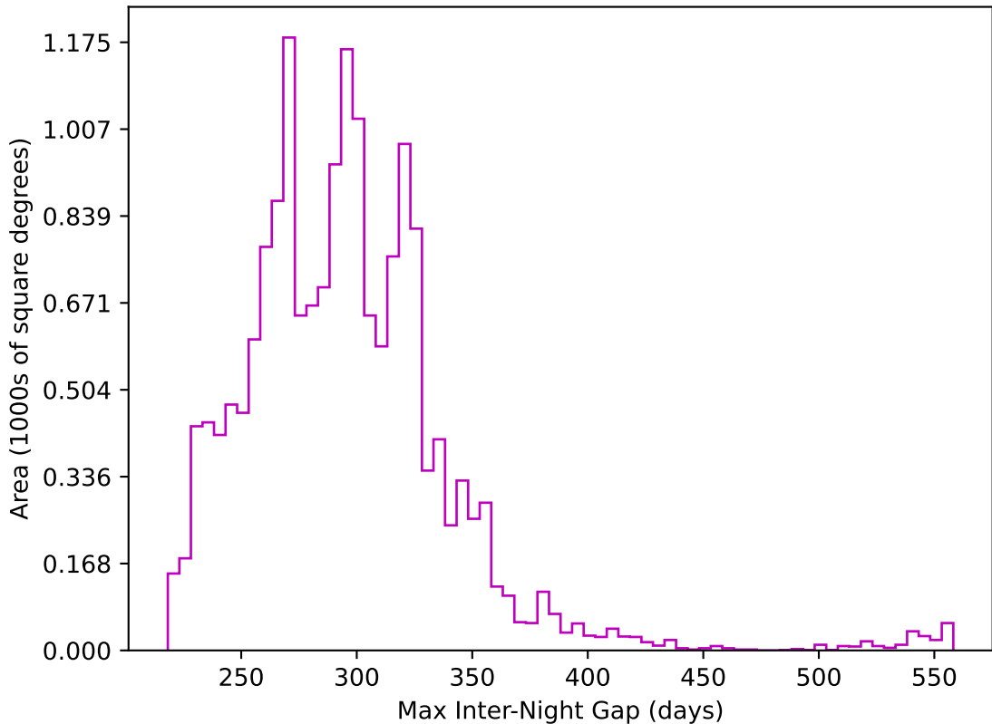
ddf_acor_sf20_lsf40_lsr50_v3.4_10yrs WFD z band: Max Inter-Night Gap
