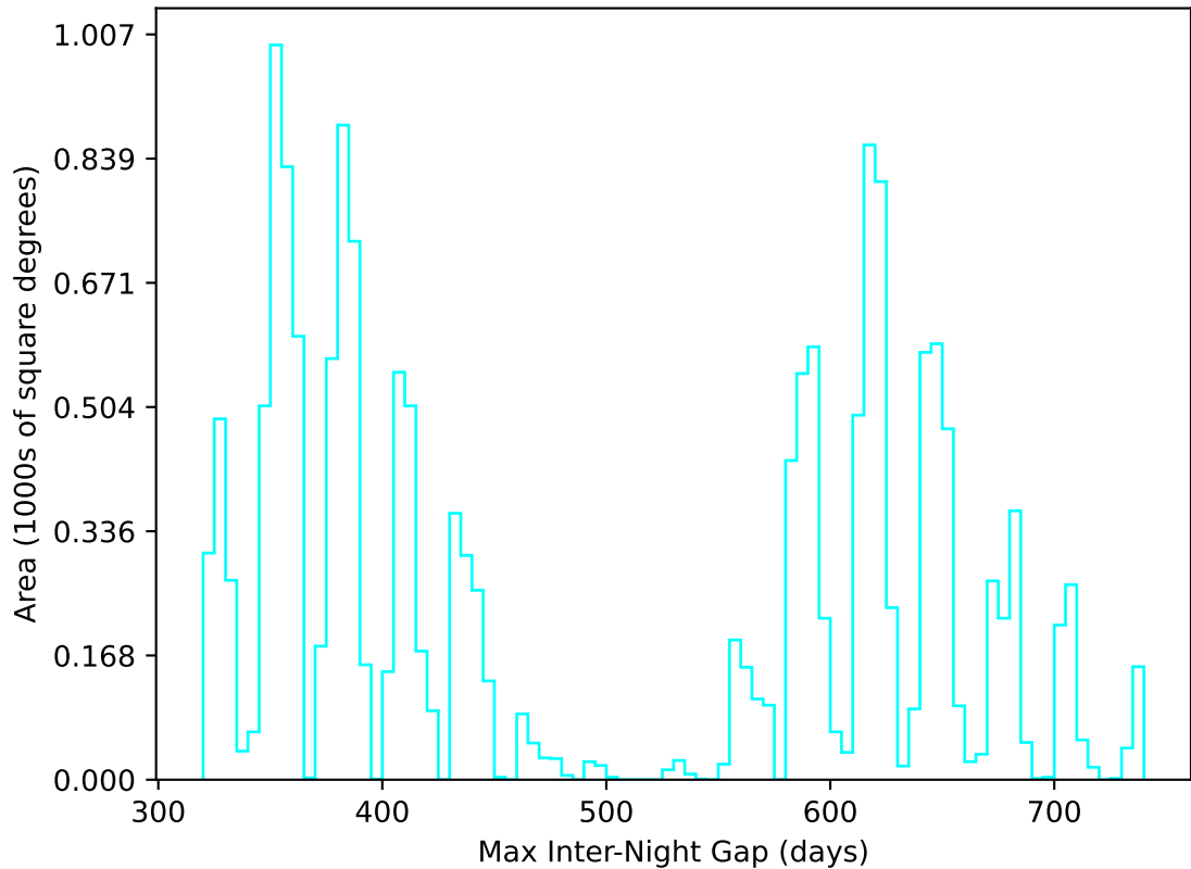
ddf_acor_sf20_lsf40_lsr50_v3.4_10yrs WFD u band: Max Inter-Night Gap
