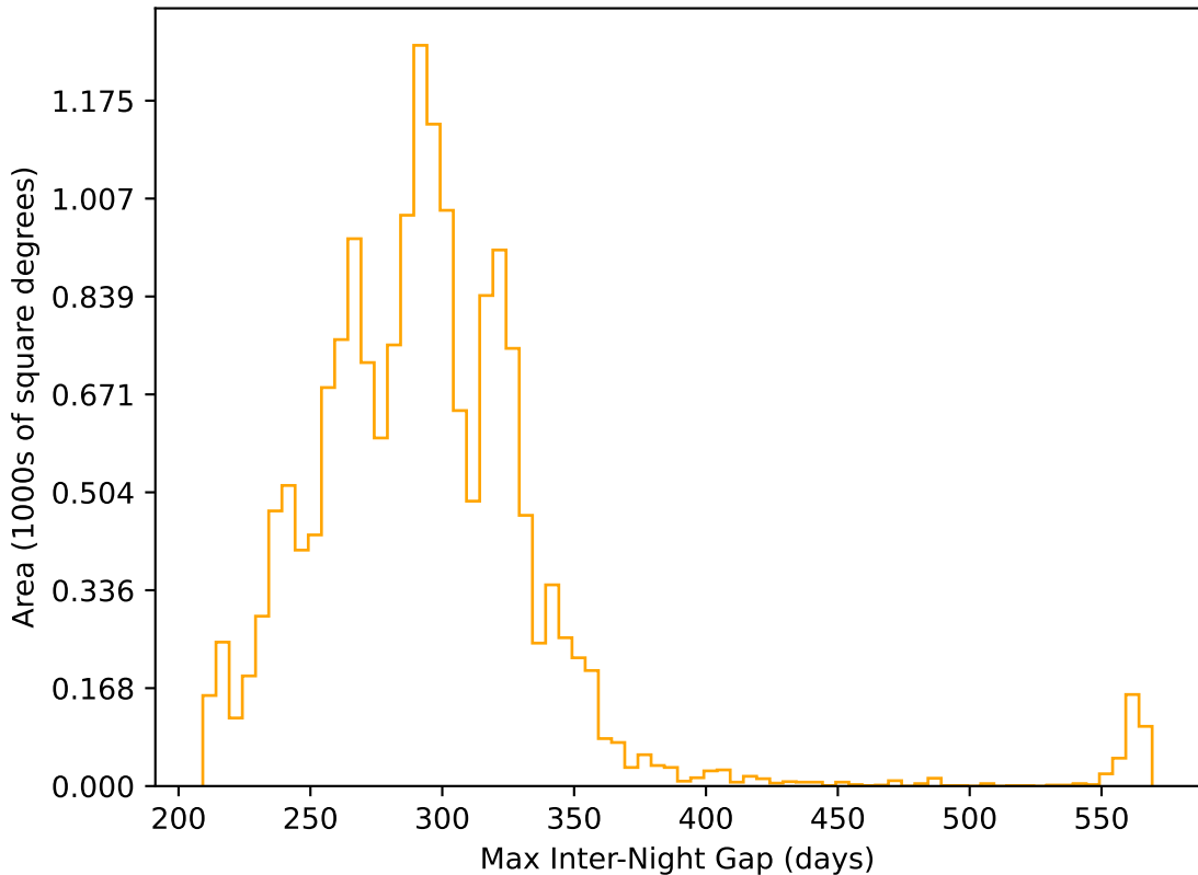
ddf_acor_sf20_lsf40_lsr50_v3.4_10yrs WFD r band: Max Inter-Night Gap
