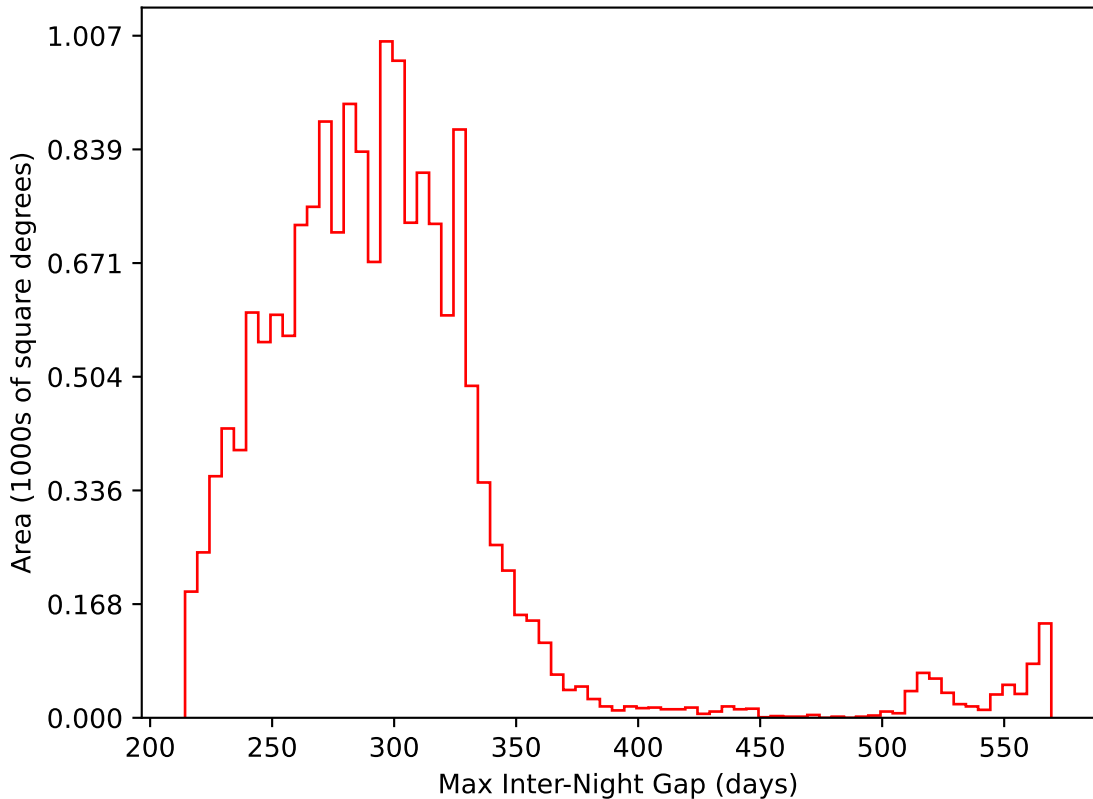
ddf_acor_sf20_lsf40_lsr50_v3.4_10yrs WFD i band: Max Inter-Night Gap
