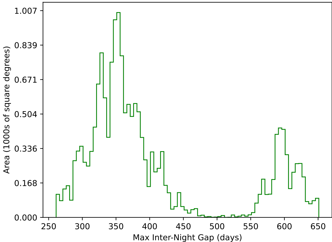
ddf_acor_sf20_lsf40_lsr50_v3.4_10yrs WFD g band: Max Inter-Night Gap
