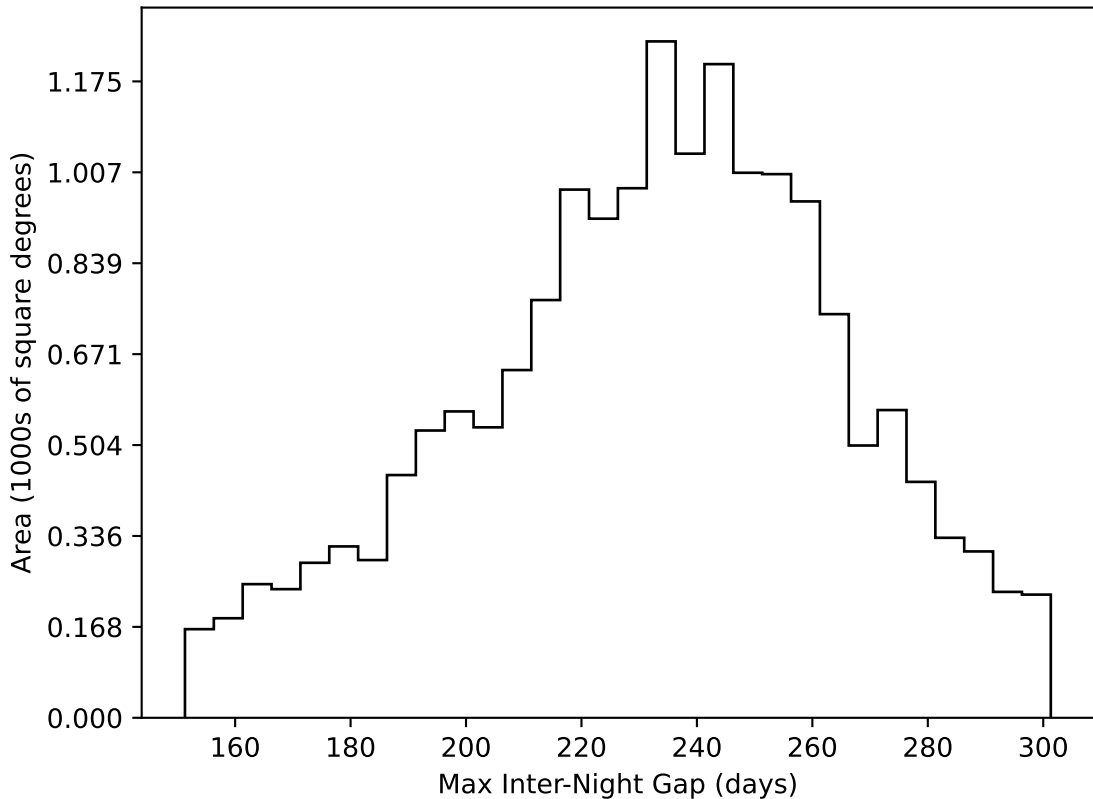
ddf_acor_sf20_lsf40_lsr50_v3.4_10yrs WFD all bands: Max Inter-Night Gap
