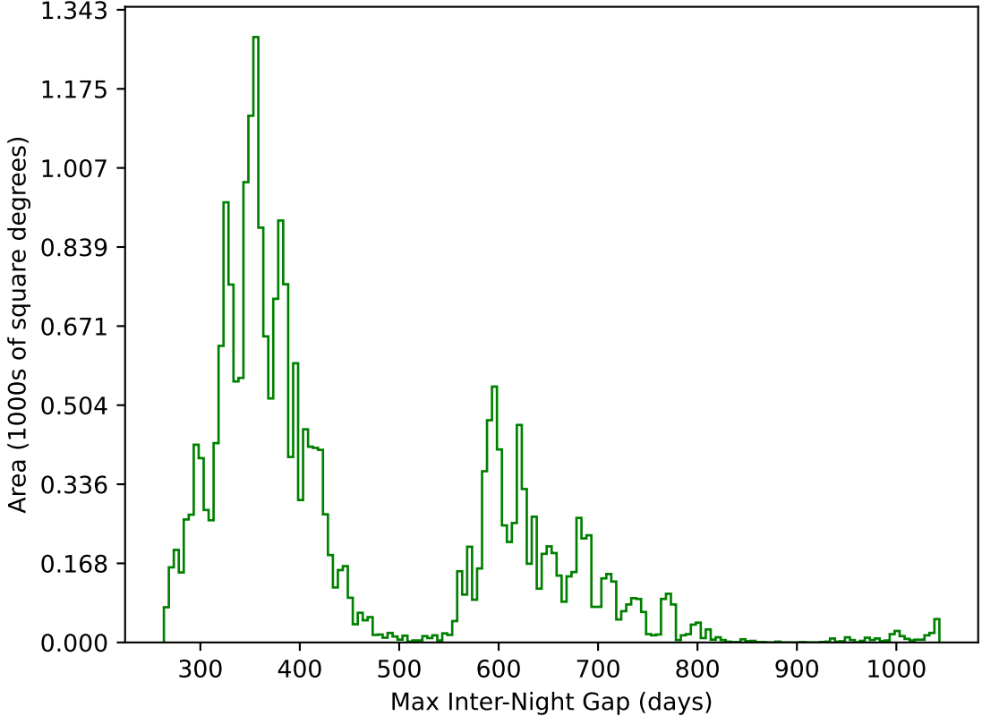
ddf_acor_sf20_ls40_lsr50_v3.4_10yrs All sky g band: Max Inter-Night Gap
