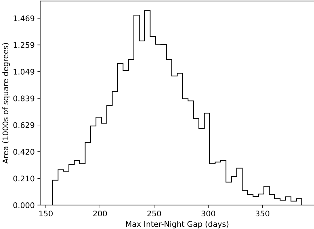
ddf_acor_sf20_lsf40_lsr50_v3.4_10yrs All sky all bands: Max Inter-Night Gap
