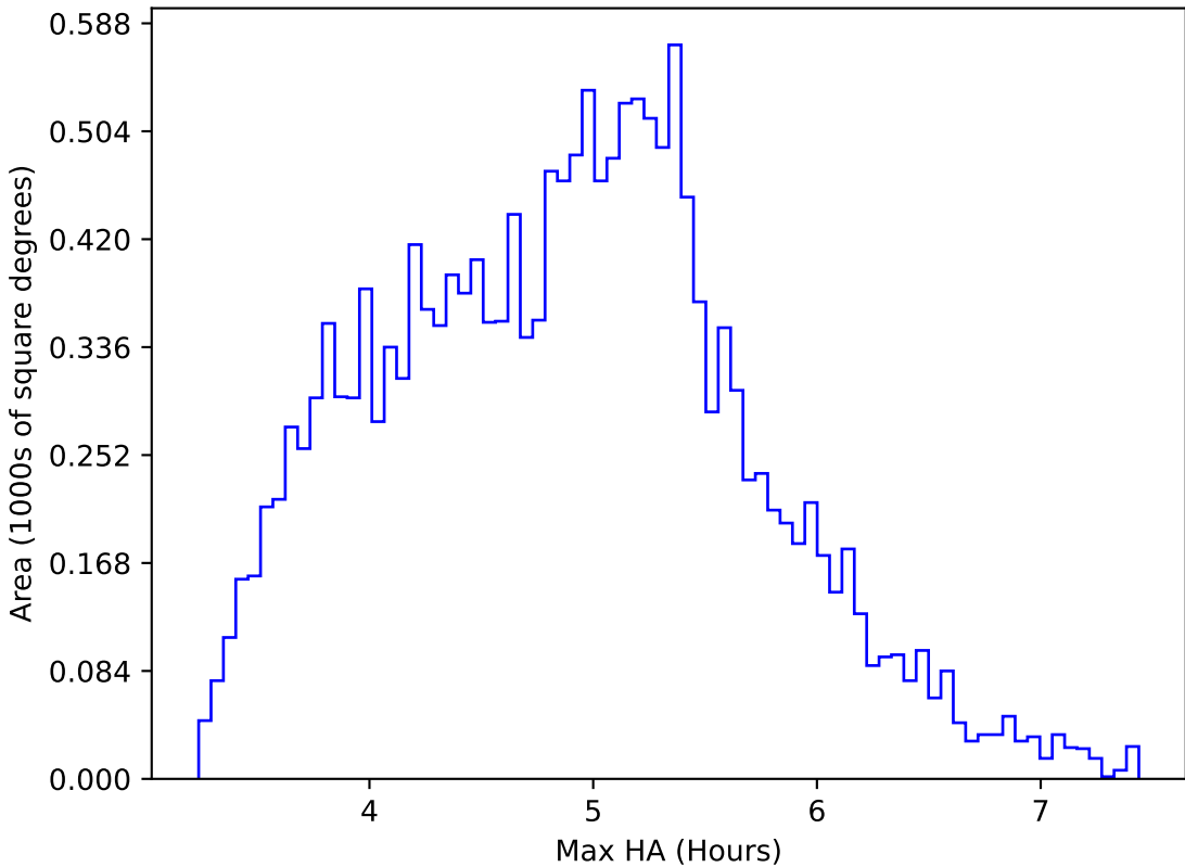
ddf_acor_sf20_lsf40_lsr50_v3.4_10yrs WFD z band: Max HA
